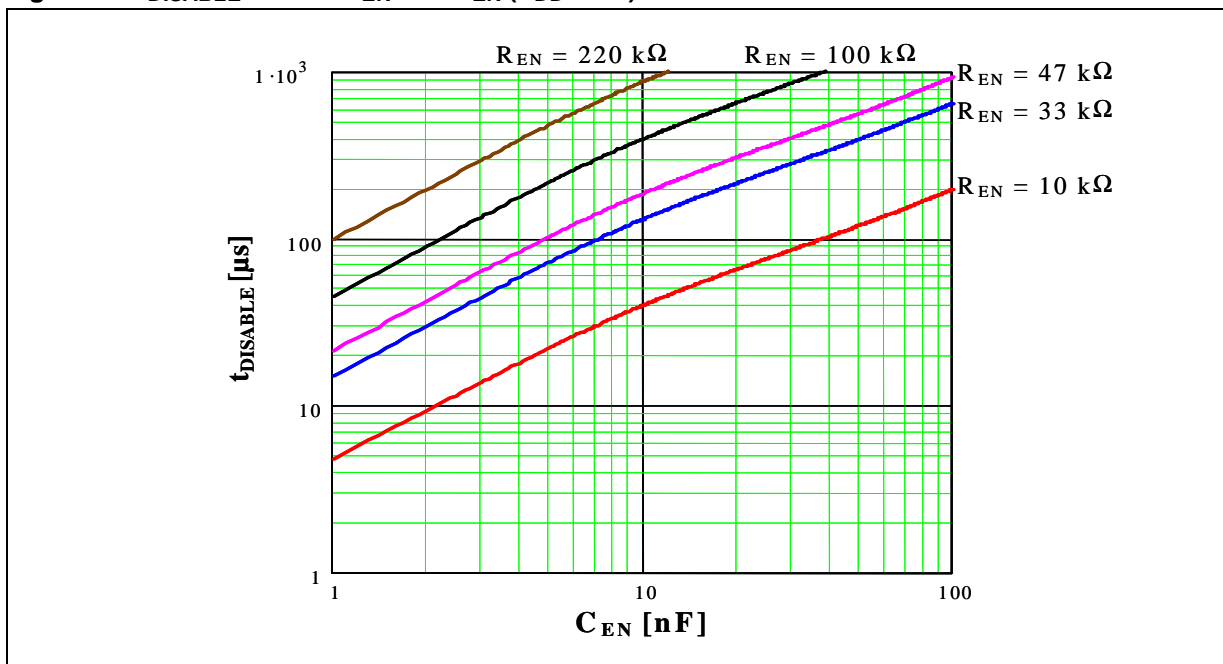
Figure 21. t_{\text{DISABLE}} versus C_{\text{EN}} and R_{\text{EN}} ( V_{\text{DD}} = 5\text{V} ).
